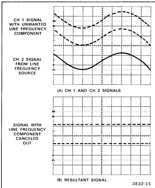
Fig. 4-3. Common-mode rejection.
