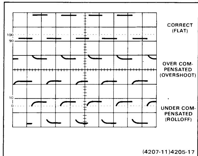
Fig. 3-2. Probe compensation.
