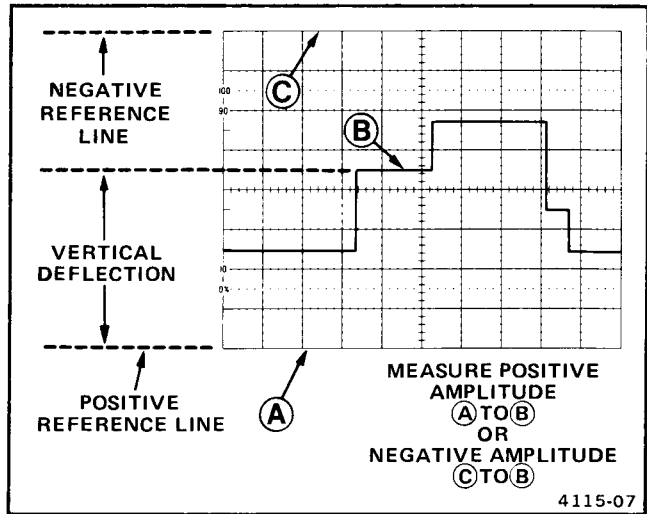
Fig. 4-1. Peak-to-peak waveform voltage.
