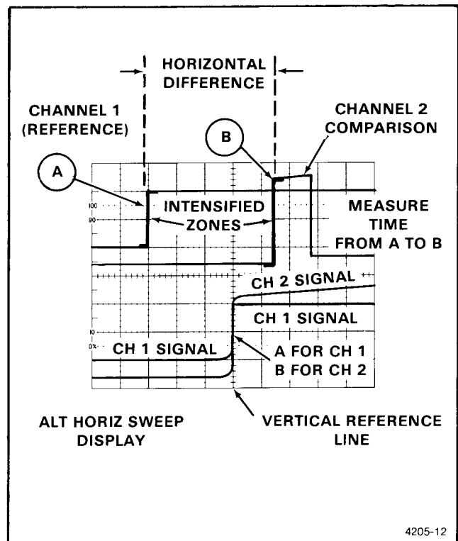
Fig. 4-8. Time difference between points on two time-related signals in nontriggered mode.
