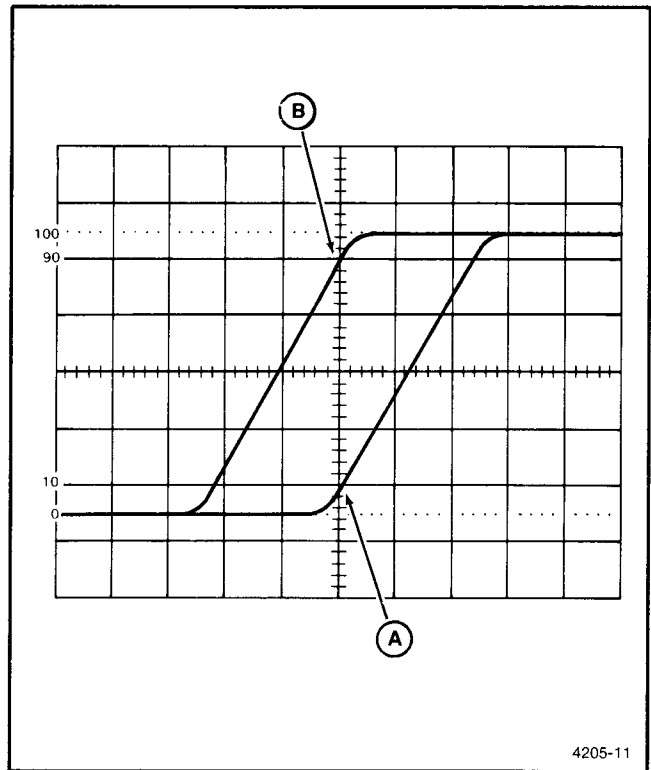
Fig. 4-7. Rise time.
