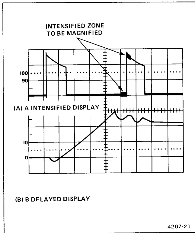
Fig. 4-5. Delayed-sweep magnification.
