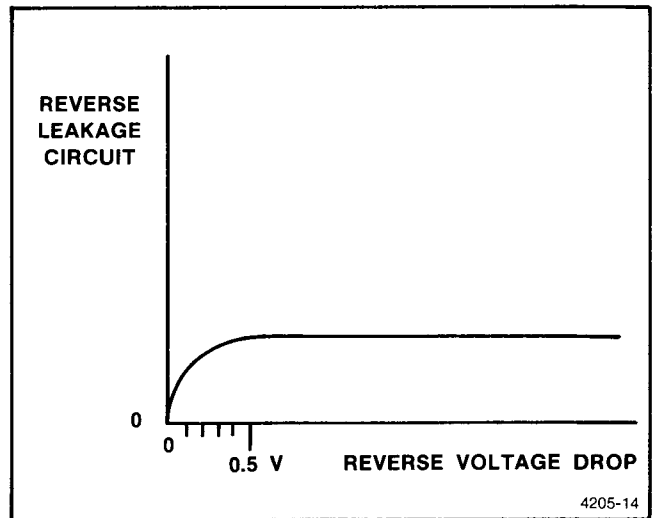
Fig. 4-10. Reverse voltage drop to reverse leakage current characteristics for typical semiconductor.
