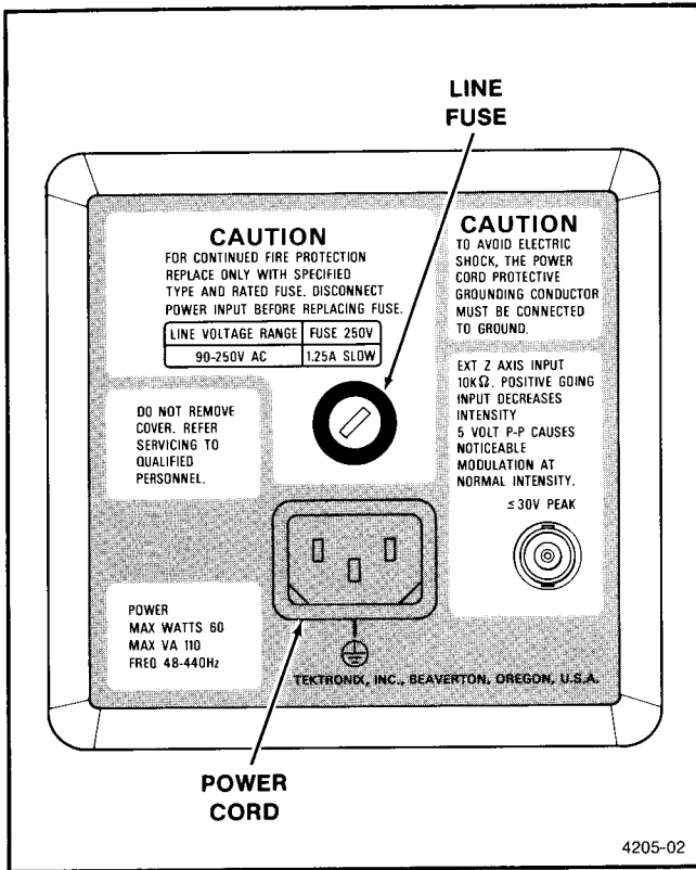
Fig. 2-2. Fuse holder and power cord connector.
