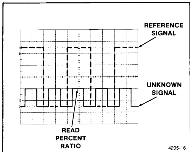
Fig. 4-4. Voltage ratios.
